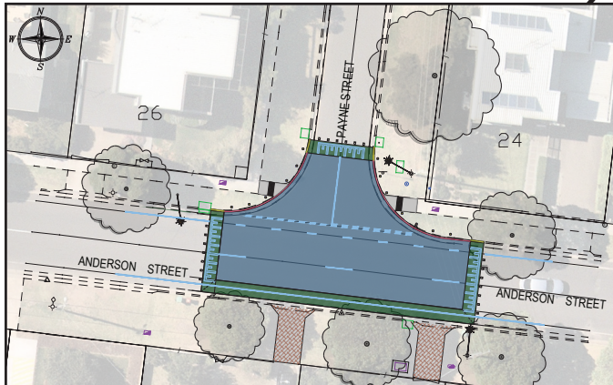
Raised intersection plan - Payne and Anderson St.
